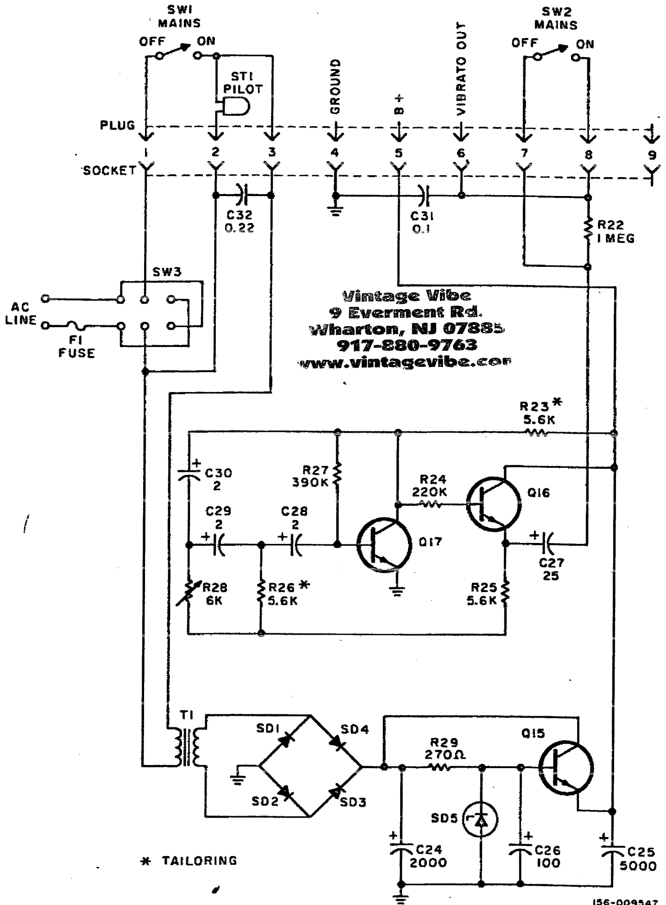
Figure 23. Power Supply Schematic
