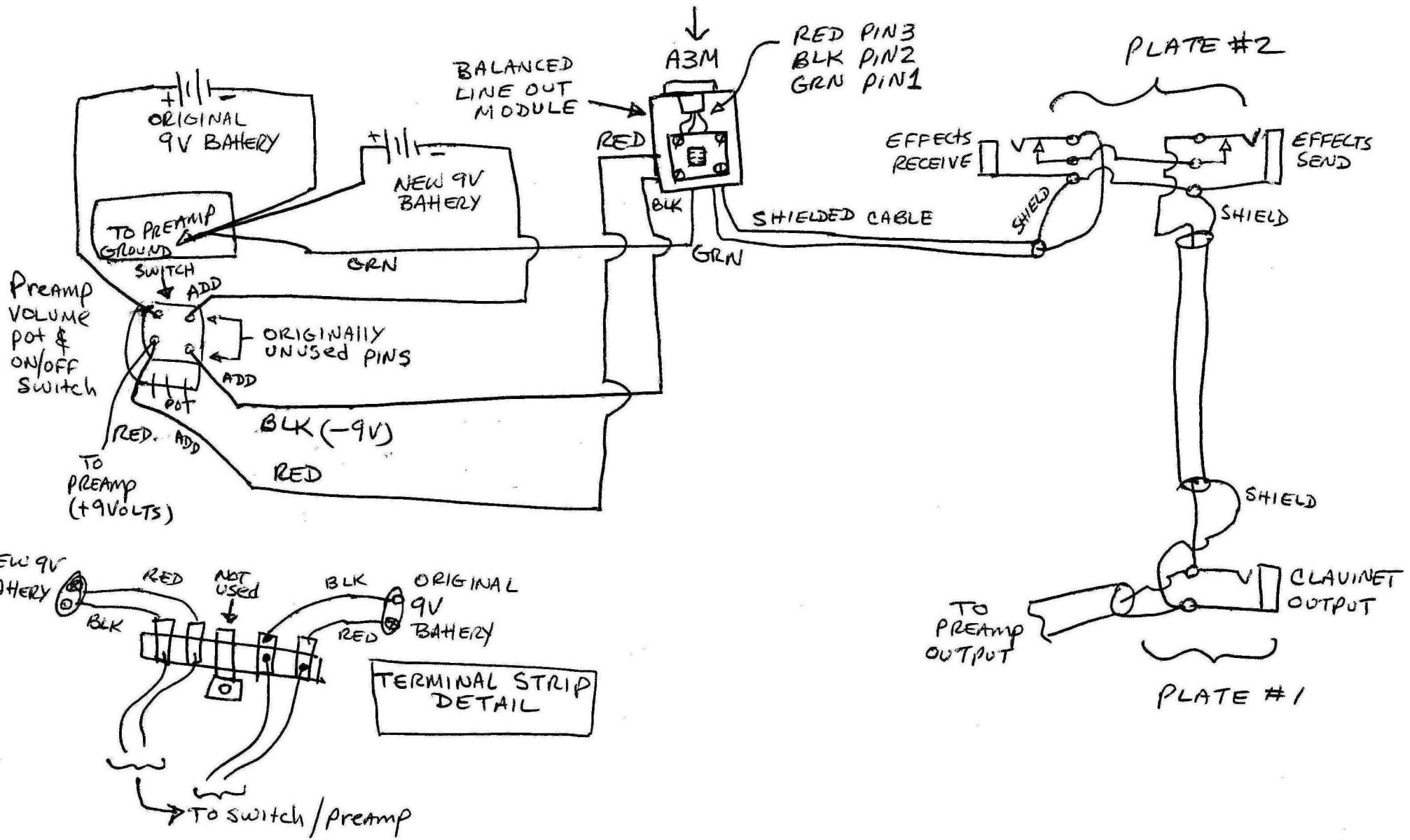
CLAVINET BALANCED LINE OUTPUT KIT Φ3-24-Φ6GH
